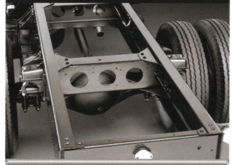
Easy Frame Assembly
